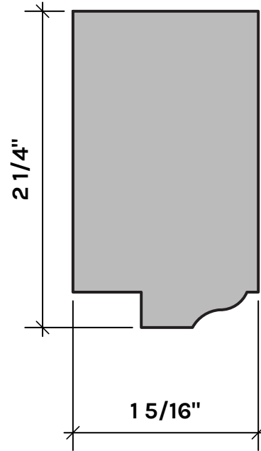
RS138SR SASH PART STOCK: POPLAR S/O: POPLAR
