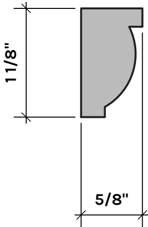
RS44SO WALL MOULDING STOCK: NONE S/O: ANY SPECIES
