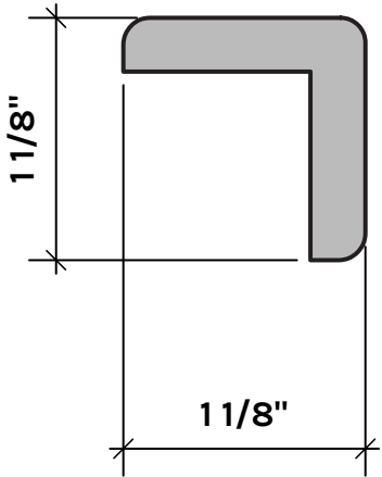
RS205C WALL MOULDING STOCK: CLEAR PINE S/O: ANY SPECIES
