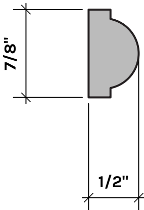
RS228SO WALL MOULDING STOCK: NONE S/O: ANY SPECIES
