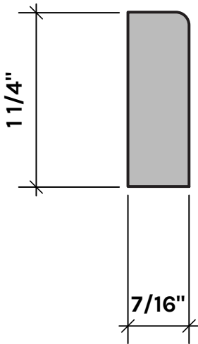
RS877C STOP STOCK: CLEAR PINE S/O: ANY SPECIES
