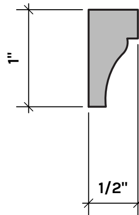
RS247SO WALL MOULDING STOCK: NONE S/O: ANY SPECIES
