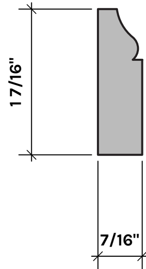
RS48SO STOP STOCK: NONE S/O: ANY SPECIES
