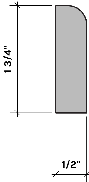
RS47SO STOP STOCK: NONE S/O: ANY SPECIES
