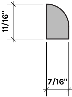
RS129P SHOE MOULD STOCK: PRIMED S/O: ANY SPECIES
