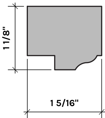
RS138PR SASH PART STOCK: POPLAR S/O: POPLAR
