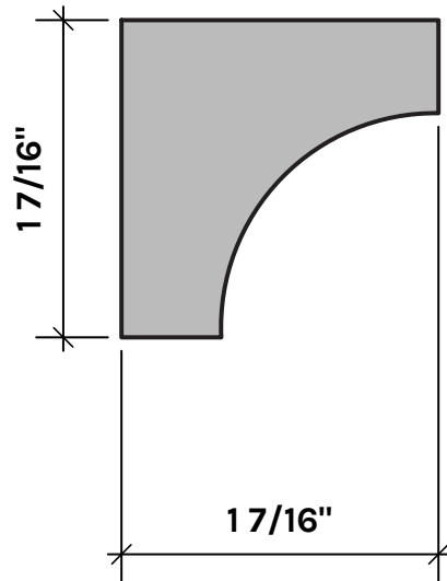
RS140SO WALL MOULDING STOCK: NONE S/O: ANY SPECIES
