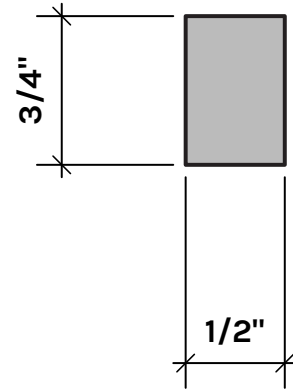
RS254C STOP STOCK: CLEAR PINE S/O: ANY SPECIES
