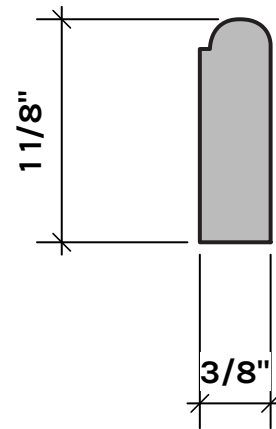
RS953C STOP STOCK: CLEAR PINE S/O: ANY SPECIES
