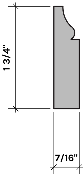
RS46SO STOP STOCK: NONE S/O: ANY SPECIES
