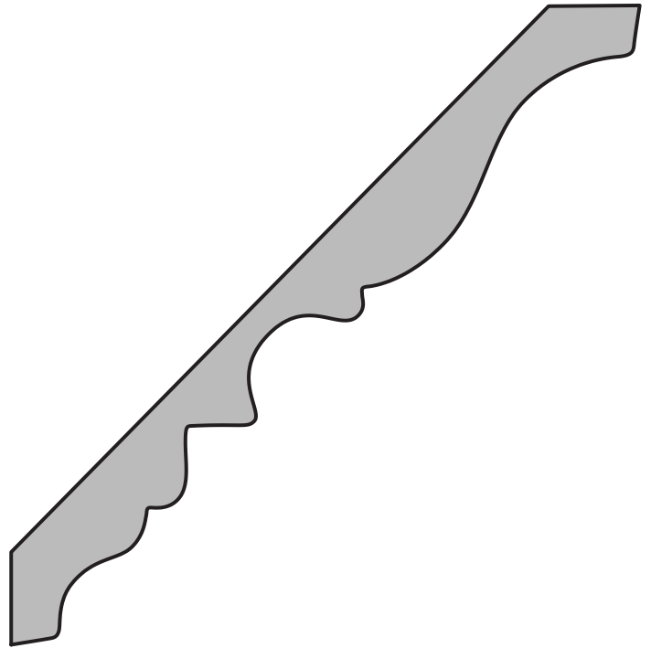
RS5047MDFSO CROWN MOULD 6 15/16" X 7 1/16" PAGE 49
