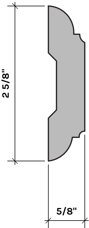
RS176SO MULLION STOCK: NONE S/O: ANY SPECIES
