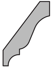
RS52P CROWN MOULD 2" X 2 3/4" PAGE 38
