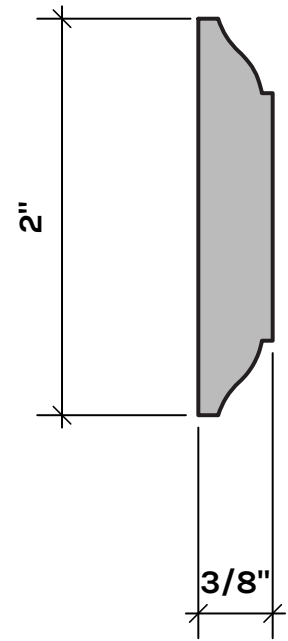
RS987 MULLION STOCK: CLEAR PINE S/O: ANY SPECIES
