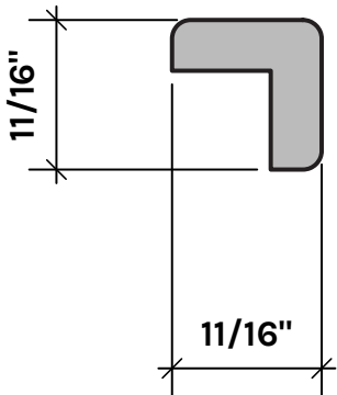
RS206C WALL MOULDING STOCK: CLEAR PINE S/O: ANY SPECIES
