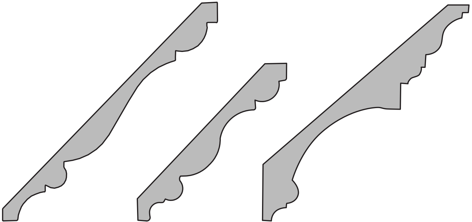
RS536MDF CROWN MOULD 7 3/16" X 7 5/16" PAGE 42
