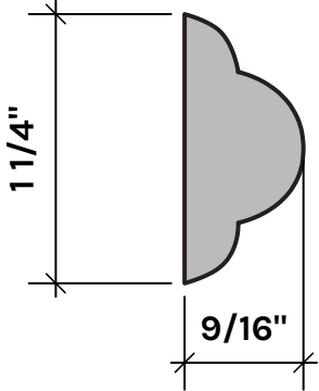
RS137P WALL MOULDING STOCK: PRIMED S/O: ANY SPECIES
