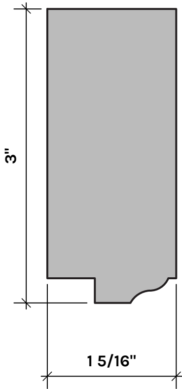
RS138BR SASH PART STOCK: POPLAR S/O: POPLAR
