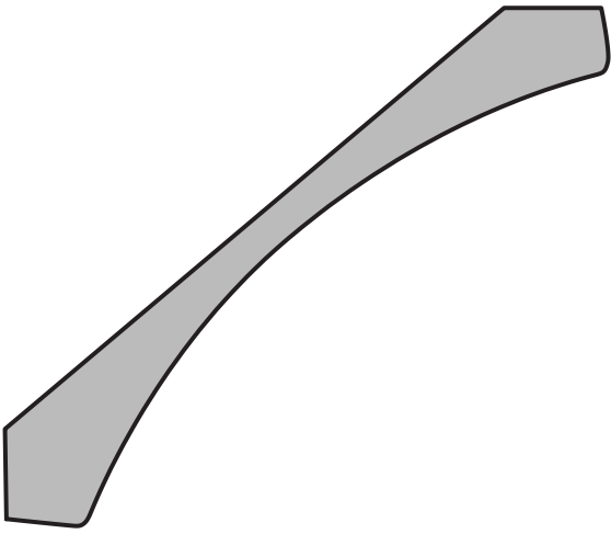
RS653MDF CROWN MOULD 5 9/16" X 4 3/4" PAGE 45
