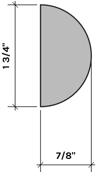
RS6S0 WALL MOULDING STOCK: NONE S/O: ANY SPECIES
