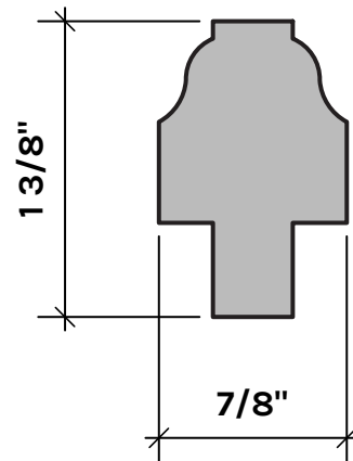
RS138MUN SASH PART STOCK: POPLAR S/O: POPLAR
