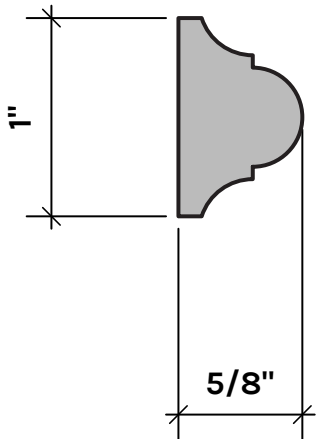
RS34SO WALL MOULDING STOCK: NONE S/O: ANY SPECIES
