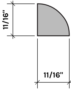
RS106P SHOE MOULD STOCK: PRIMED S/O: ANY SPECIES
