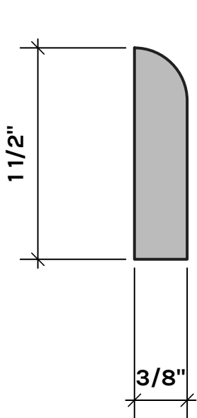
RS46SO STOP STOCK: NONE S/O: ANY SPECIES
