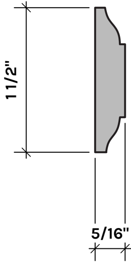
RS985C MULLION STOCK: CLEAR PINE S/O: ANY SPECIES
