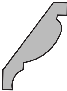
RS259SO CROWN MOULD 2 1/8" X 2 7/8" PAGE 48
