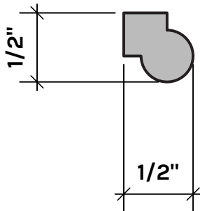
RS244SO WALL MOULDING STOCK: NONE S/O: ANY SPECIES
