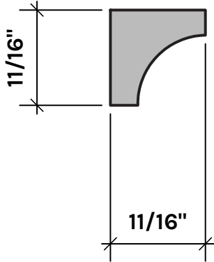
RS100C WALL MOULDING STOCK: CLEAR PINE S/O: ANY SPECIES
