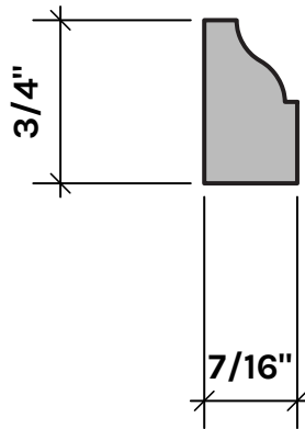
RS941C STOP STOCK: CLEAR PINE S/O: ANY SPECIES
