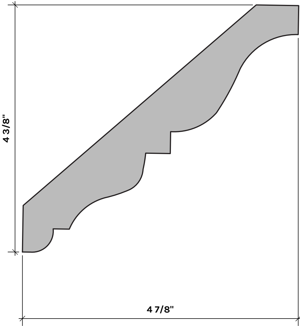
RS230SO CROWN MOULD STOCK: NONE S/O: ANY SPECIES
